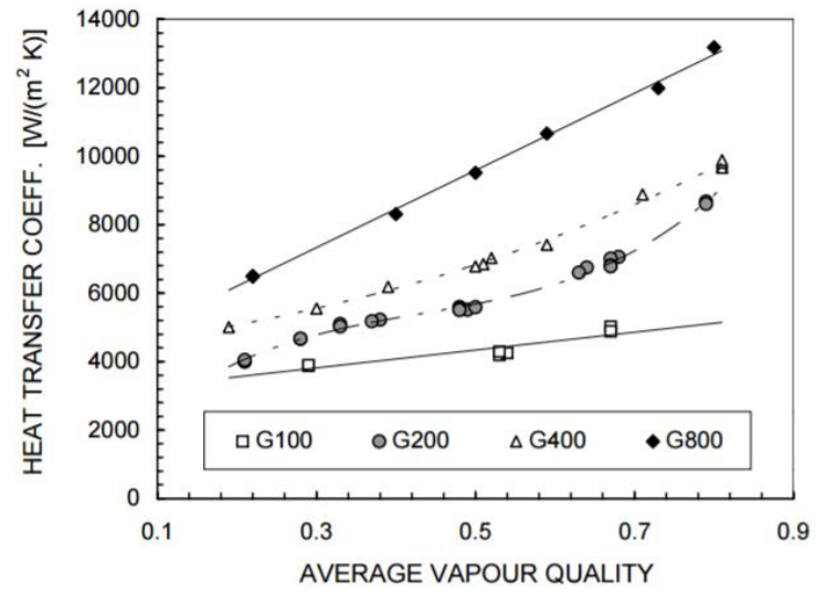
Figure 2: Heat transfer coefficients for R134a at 40°C saturation temperature. G is mass velocity [kg/(m 2 s)].
